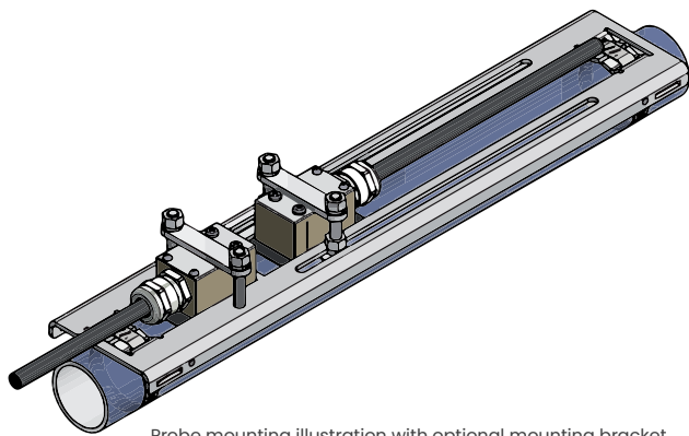
Probe mounting illustration with optional mounting bracket
